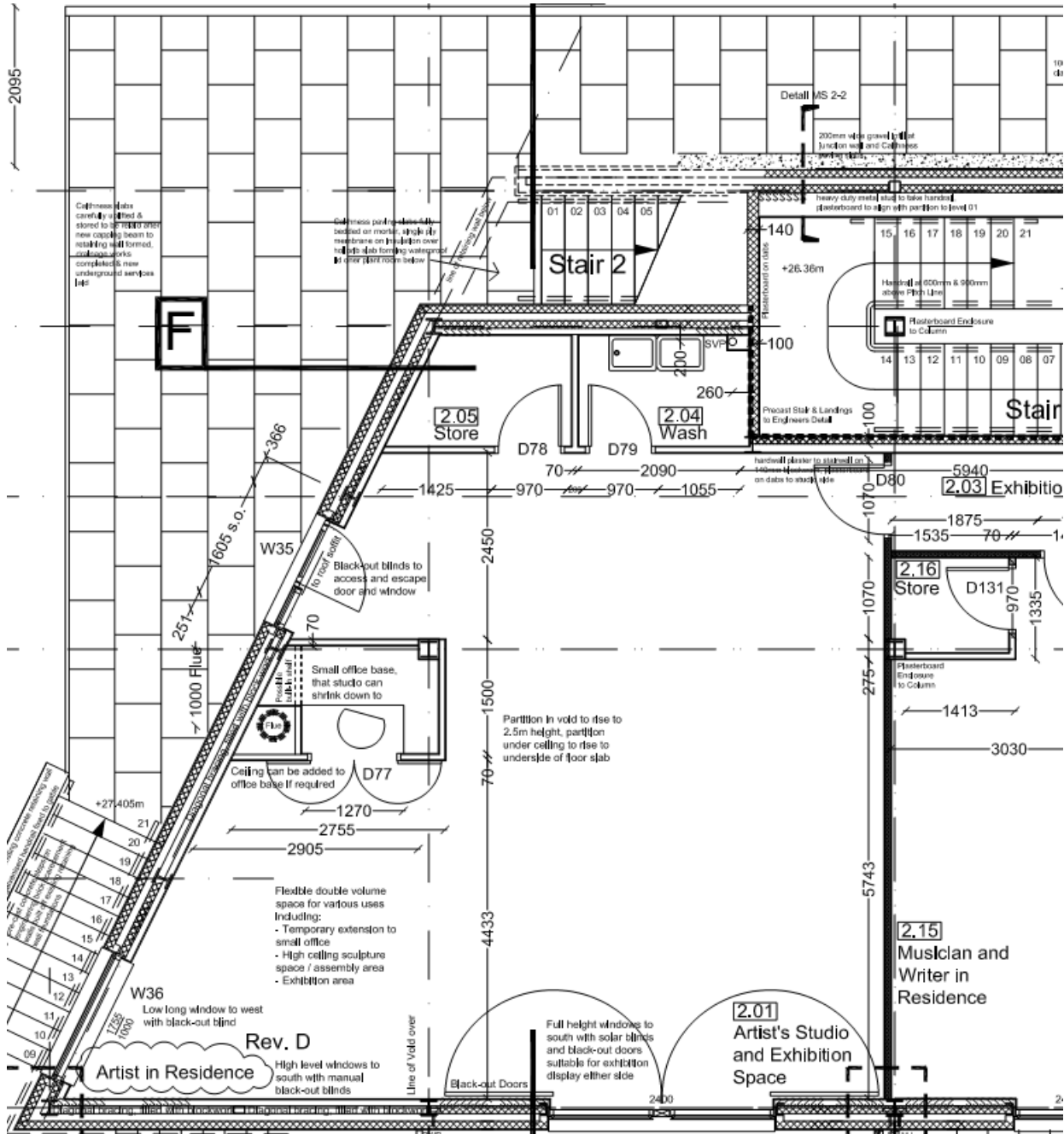
Plan of Artist's Studio at Sabhal Mòr Ostaig
